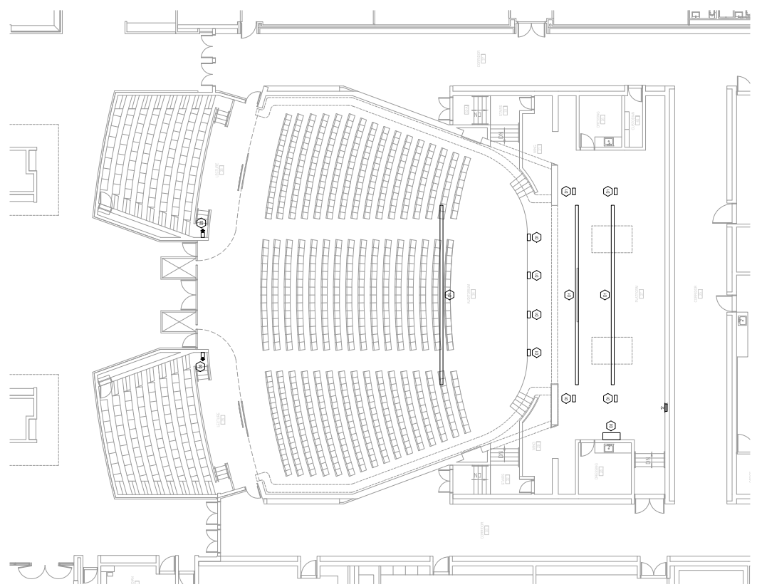
ELECTRICAL DEMOLITION PLAN AUDITORIUM AREA 1/4" = 1'-0"
